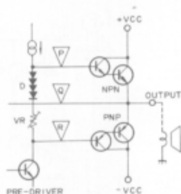
Fig. 4 Normal class B SEPP power stage
