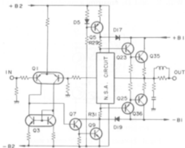
Fig. 3 Basic circuit of power amplifier
